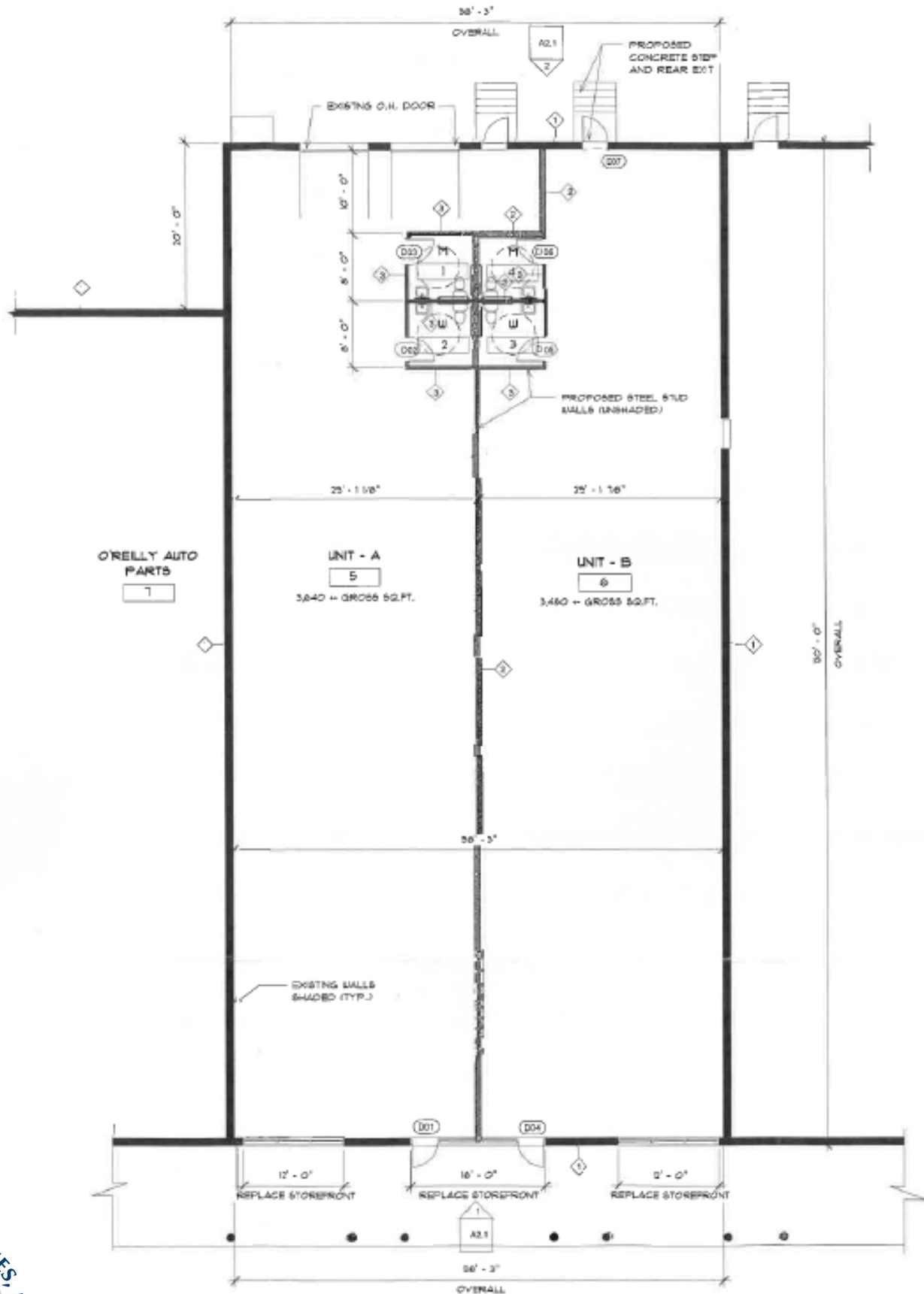
① Level 1 - PROPOSED 1/8" = 1'-0"
